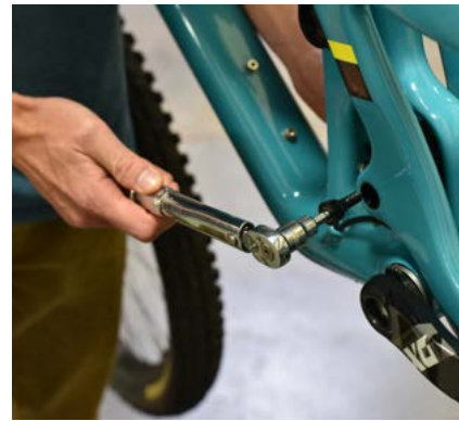
07. Install the Main Pivot Collet Wedge and *Torque to 14 Nm.
