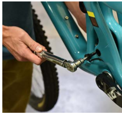
07. Install the Main Pivot Collet Wedge and *Torque to 14 Nm.
